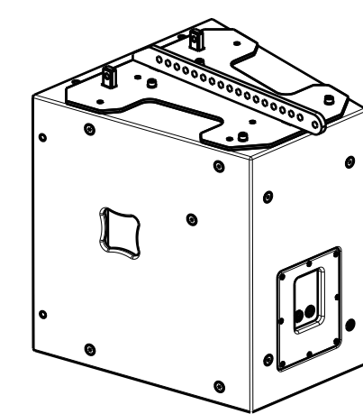
Mounting example1 Single (SCALE 14:1)
