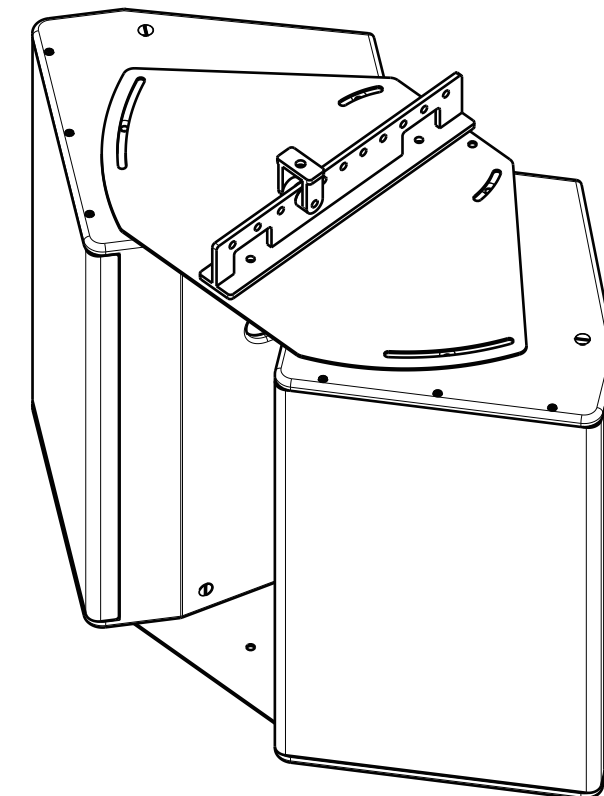
Mounting example 2 CP-XY15DF1 + CP-XY15AB1
