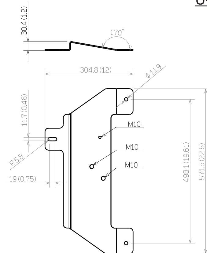
SIDE PLATE-L
