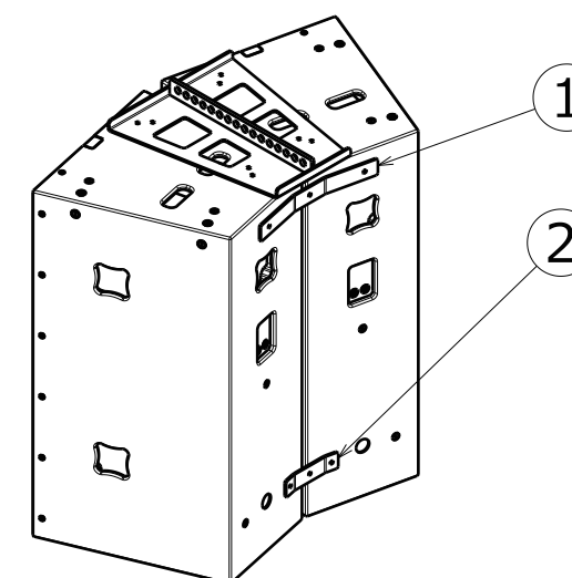
Mounting example2 Dual (SCALE 16:1)
