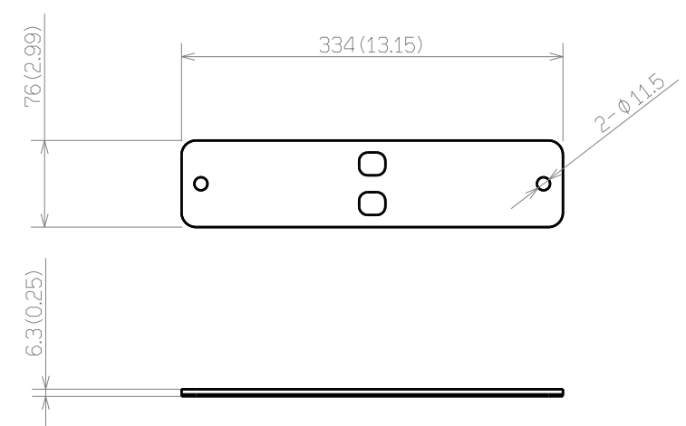
REAR PLATE
