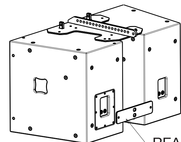
Mounting example2 Dual (SCALE 14:1)
