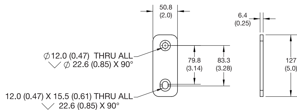
① CONNECTOR PLATE
