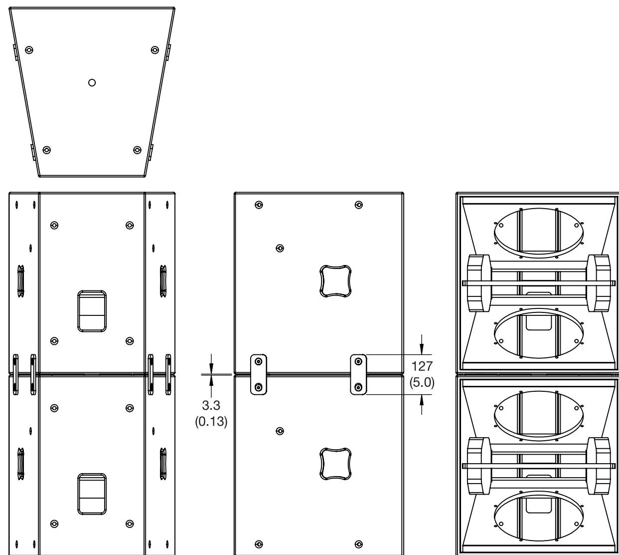
Mounting example (SCALE 12:1)
