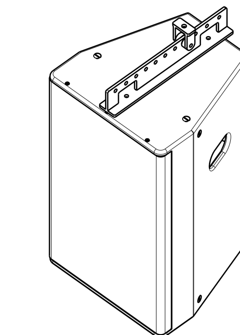
Mounting example 2 CP-XY15AB1 only
