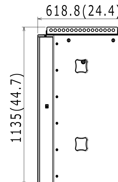
Mounting example2 Dual (SCALE 16:1)
