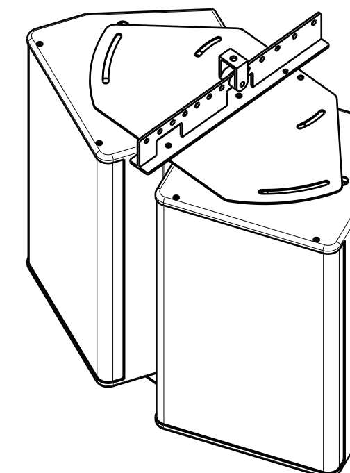
Mounting example 2 CP-XY12DF1 + CP-XYAB1
